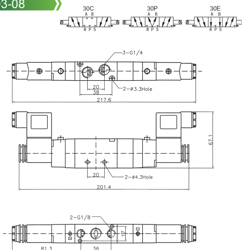
XG4303-08
