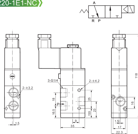
XG-220-1E1-NC
