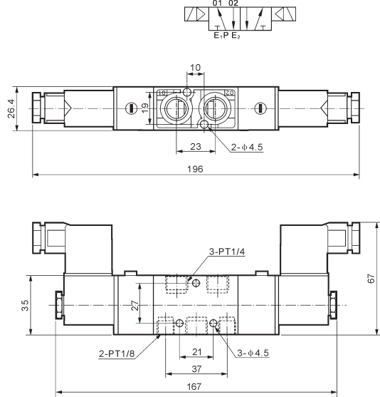
XG-260-4E2
