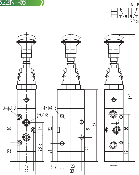
XG522N-R6
