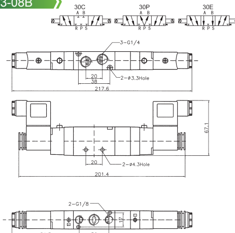
XG4303-08B
