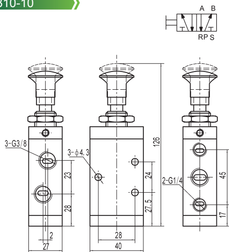
4R310-10
