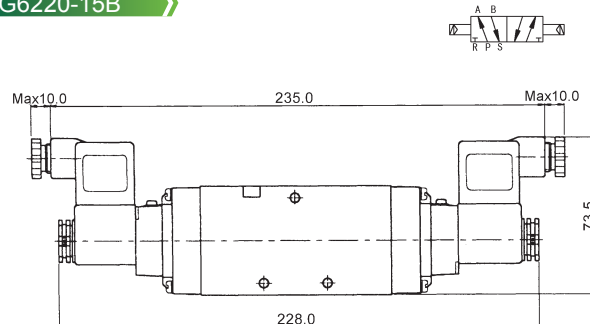
XG6220-15B
