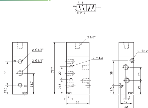
4A210-08
