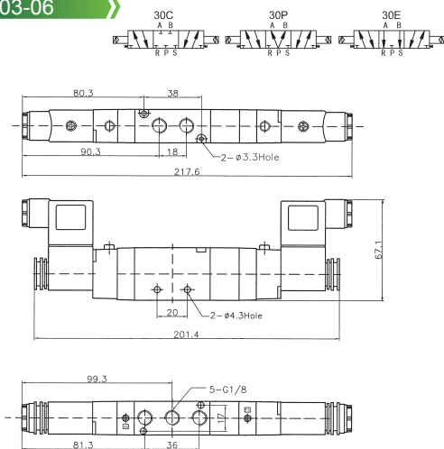
XG4303-06
