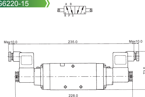
XG6220-15
